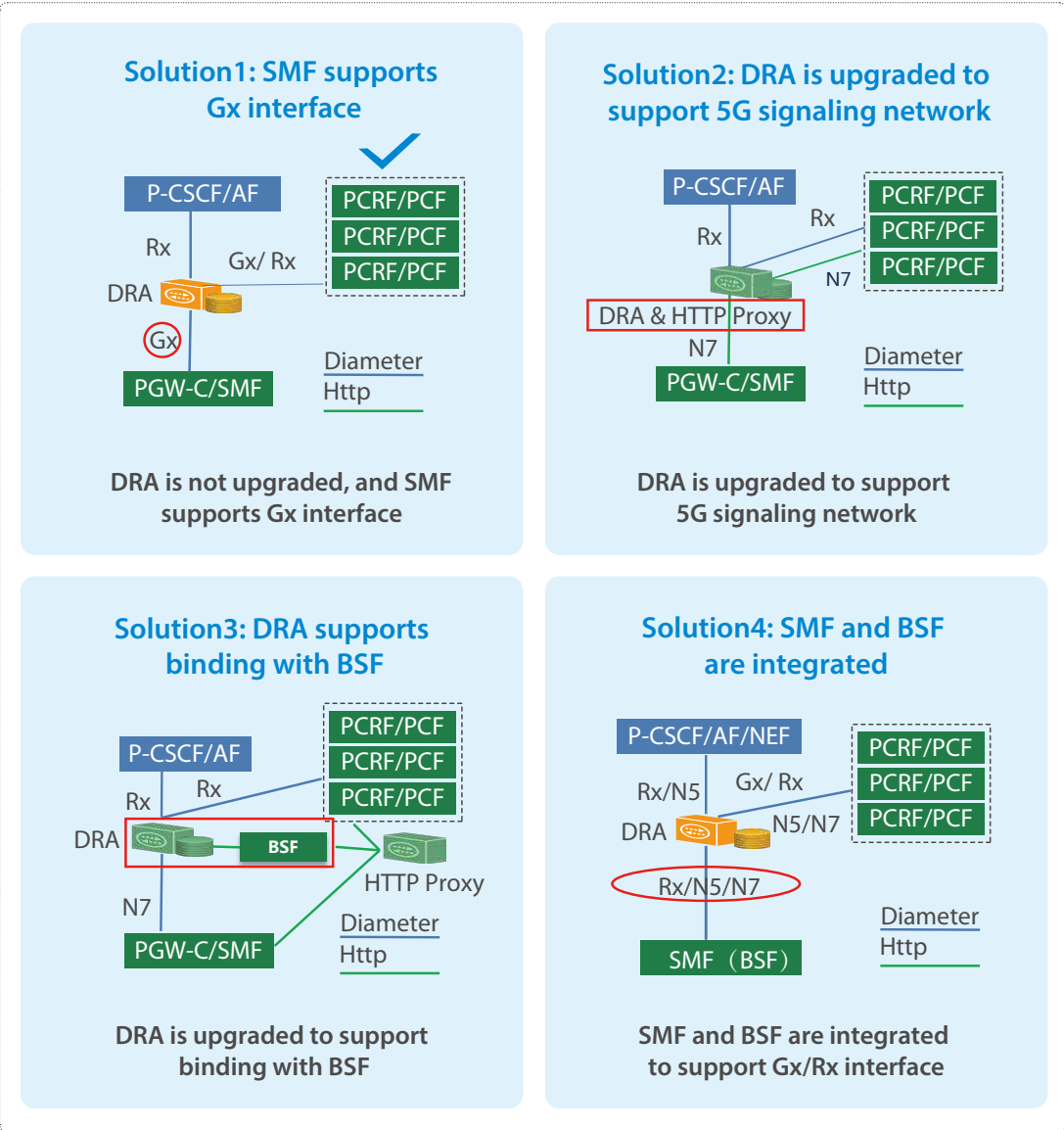
Figure 3-2 Four Session Binding Methods
