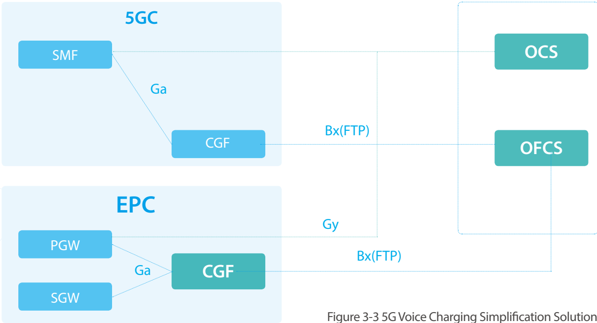
Figure 3-3 5G Voice Charging Simplification Solution
